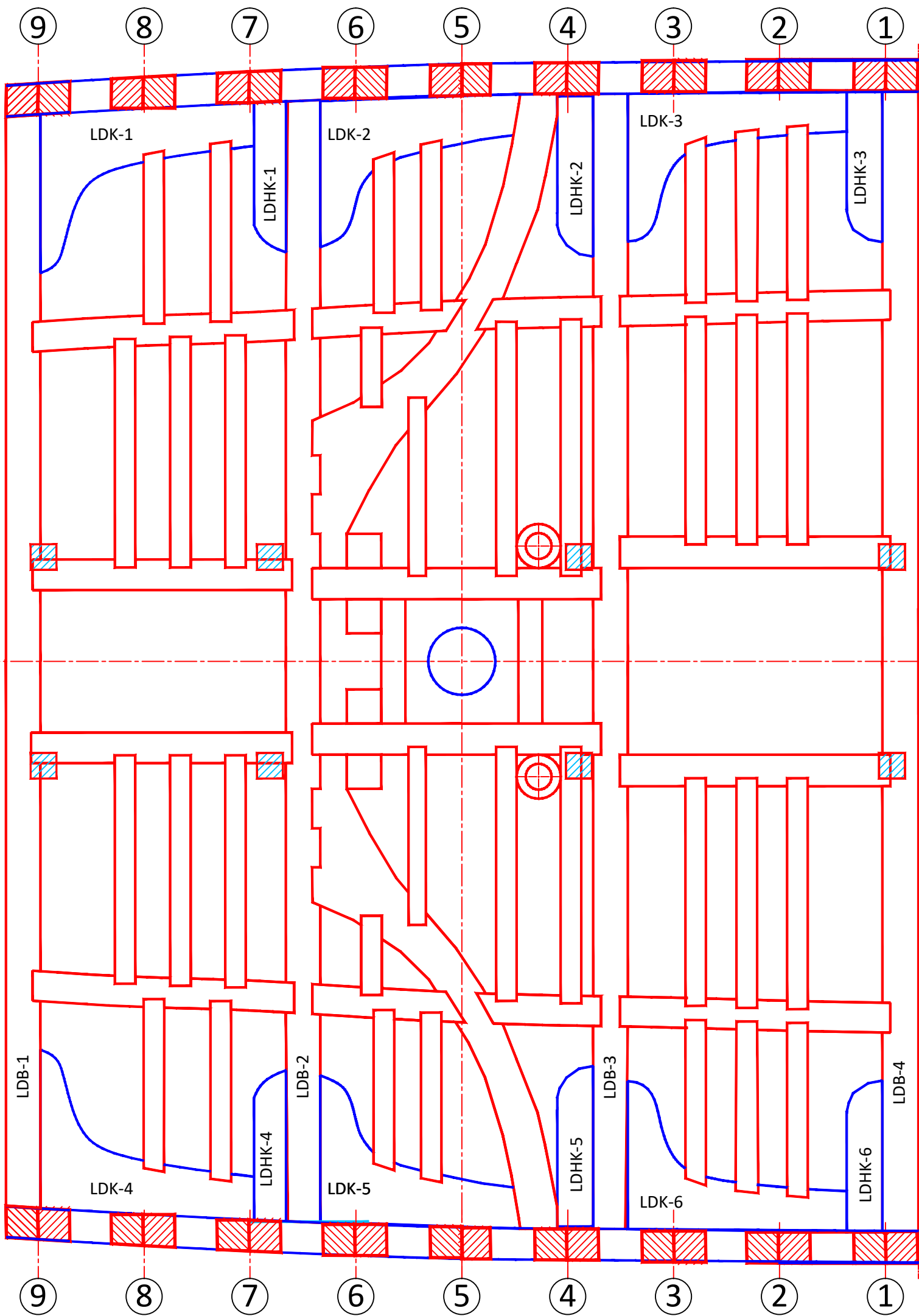
Lower Deck Framing Plan
