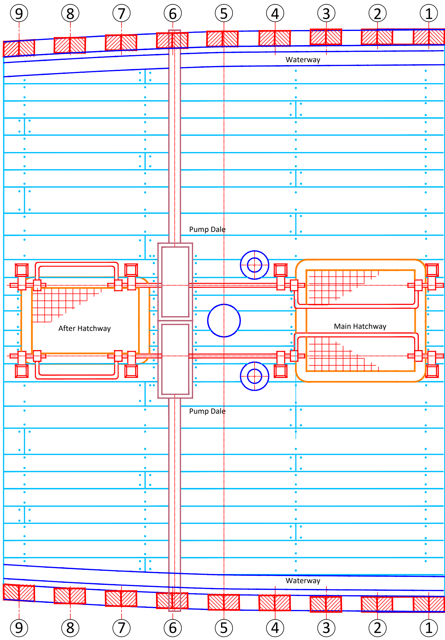
Lower Deck Plan
