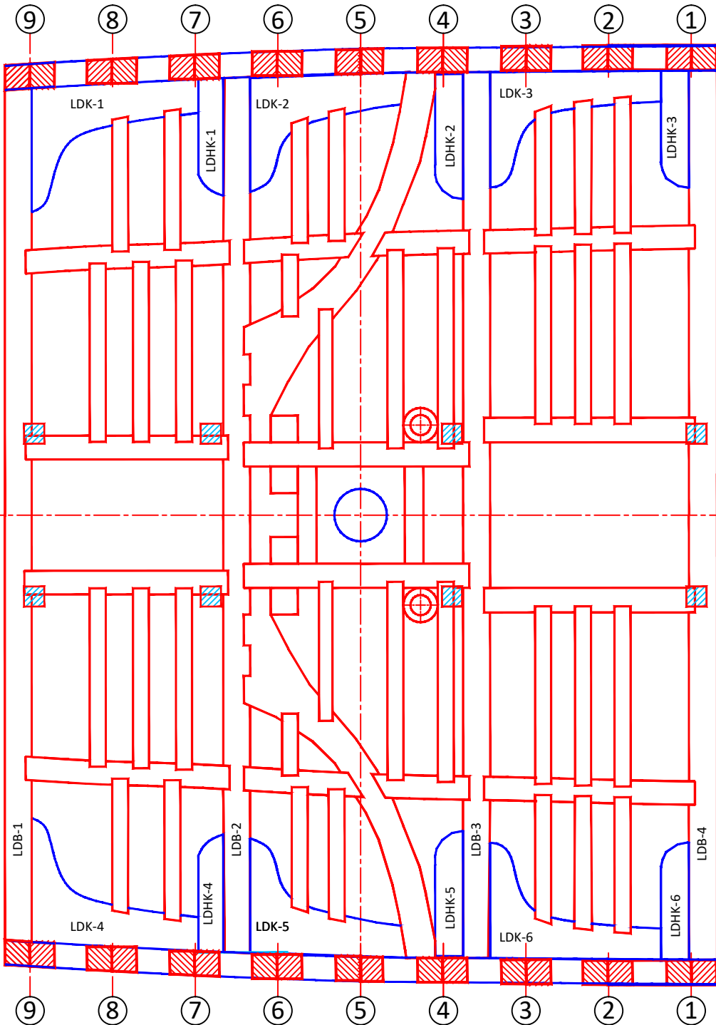
Lower Deck Framing Plan
