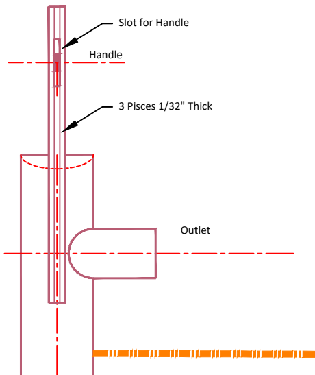
Handel Support Detail Not to Scale
