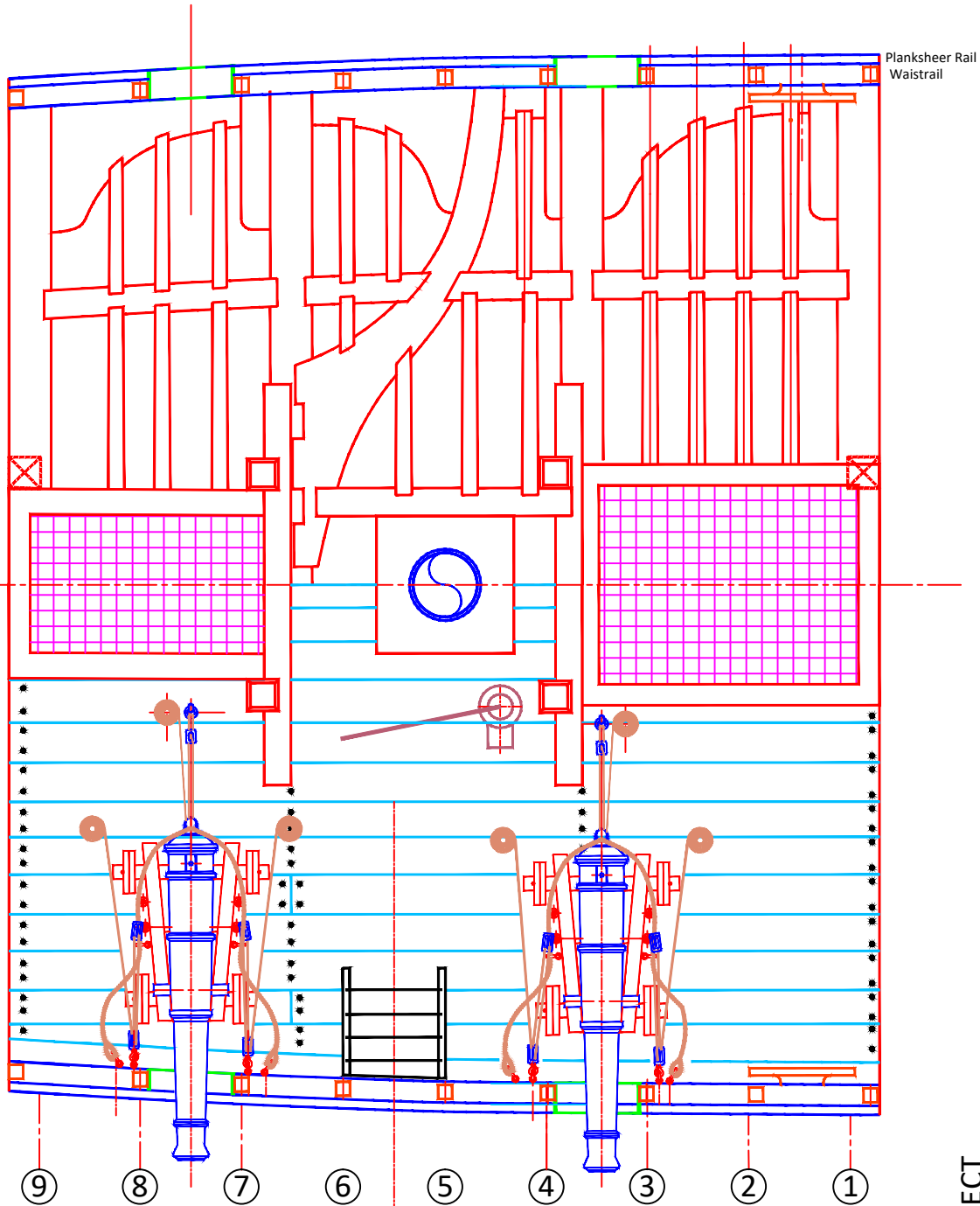
Main Deck Plan Half Planking 2 Guns
